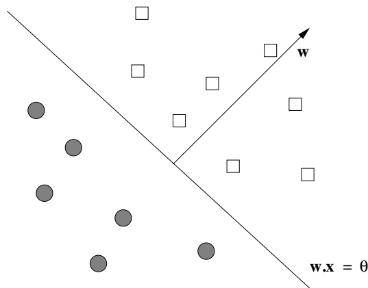
Figure 12.4 A perceptron divides a space by a hyperplane into two half-spaces
