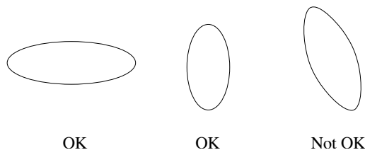
Figure 7.10 The clusters in data for which the BFR algorithm may be used can have standard deviations that differ along different axes, but the axes of the cluster must align with the axes of the space
