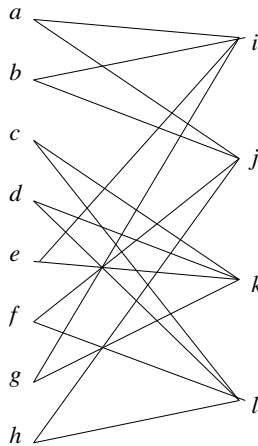
Figure 2.10 Input-output relationship for matrix multiplication
