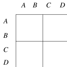
Figure 5.13 A four-node graph is divided into four 2 \times 2 blocks
