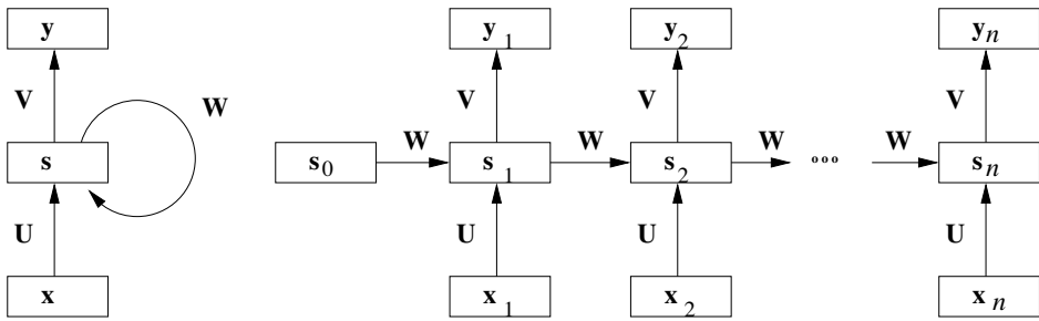
(a) The basic unit of an RNN.
